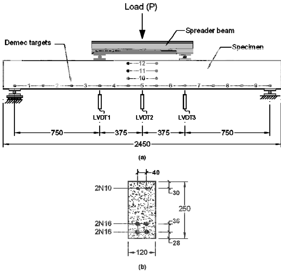
Figure 1: Details of (a) Test Arrangement, (b) Cross Section.
